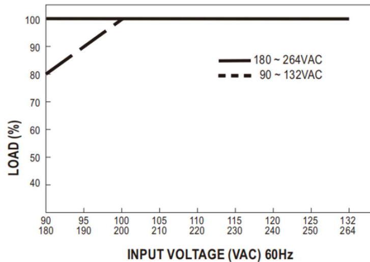
Figure 2) AC Input Voltage Derating / Output Load Derating Versus Input Voltage
